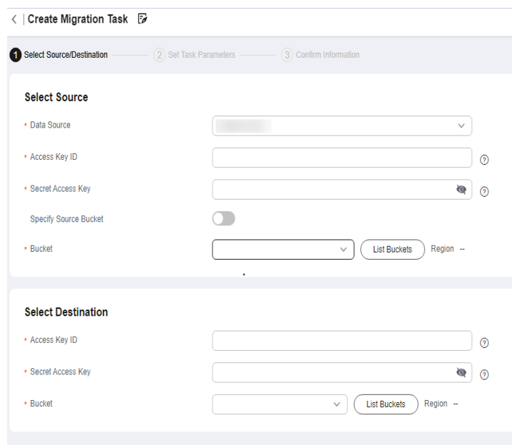
Figure 4-4 Select Source/Destination
