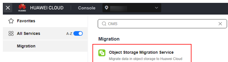
Figure 4-2 Choosing OMS
