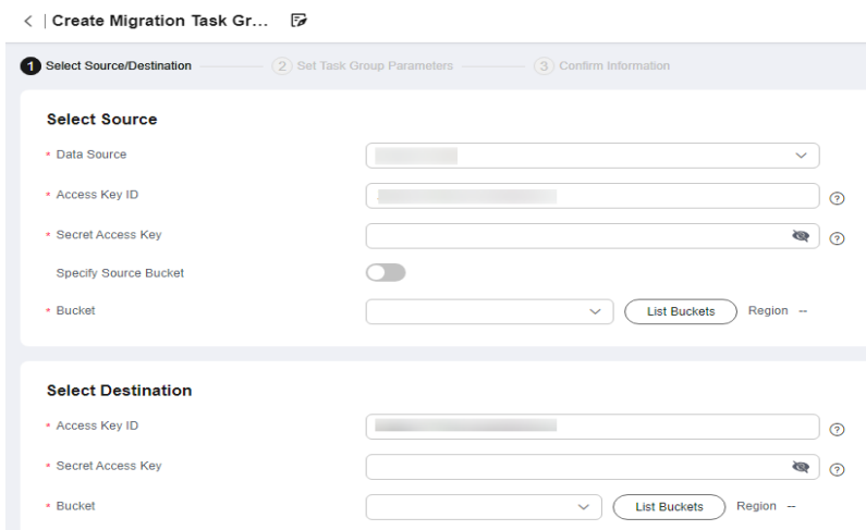
Figure 5-158 Select Source/Destination
