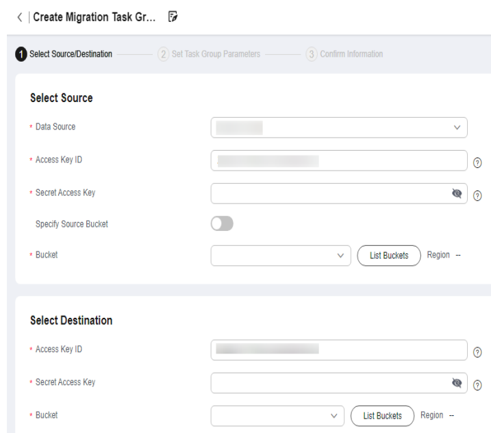
Figure 5-14 Select Source/Destination
