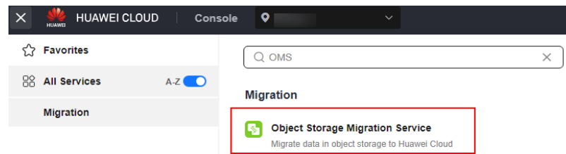
Figure 5-38 Choosing OMS
