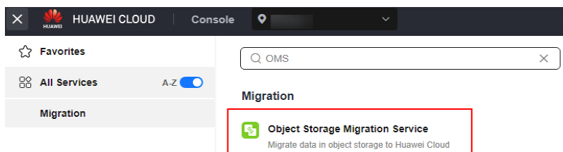
Figure 5-64 Choosing OMS
