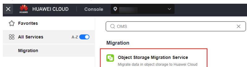
Figure 5-156 Choosing OMS
