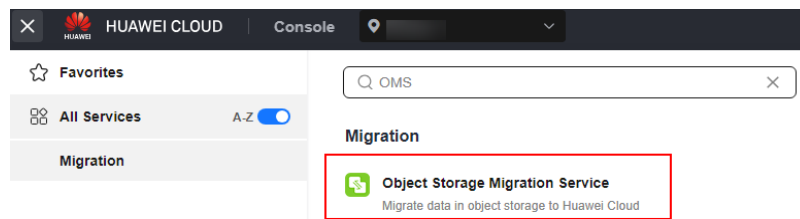
Figure 5-12 Choosing OMS
