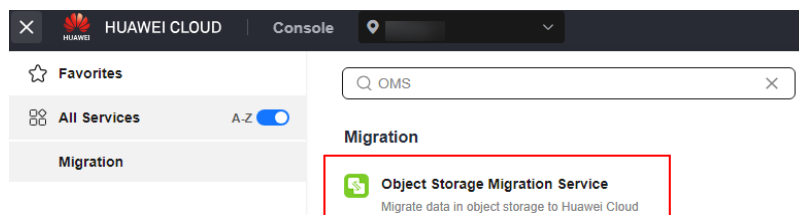
Figure 5-148 Choosing OMS
