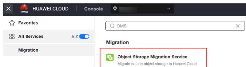
Figure 5-162 Choosing OMS
