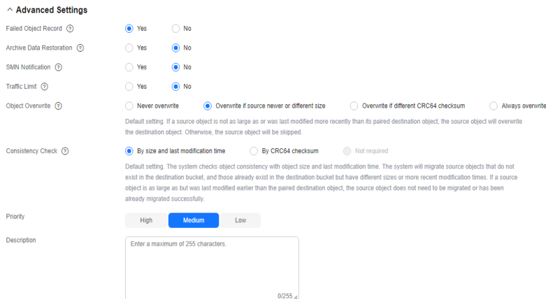
Figure 5-10 Advanced settings
