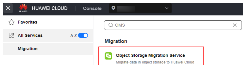
Figure 5-30 Choosing OMS
