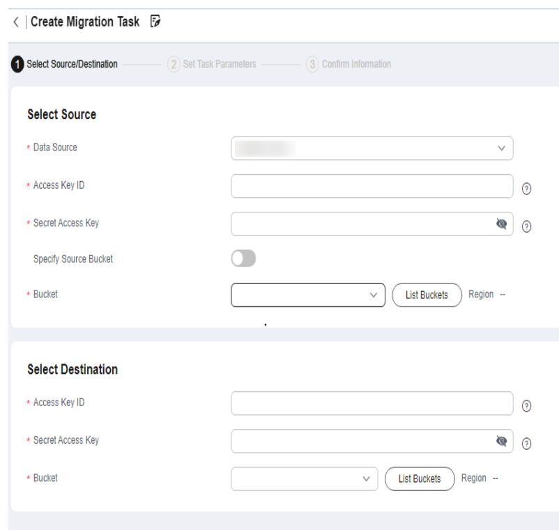
Figure 5-40 Select Source/Destination
