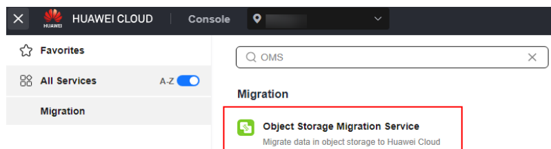
Figure 5-114 Choosing OMS
