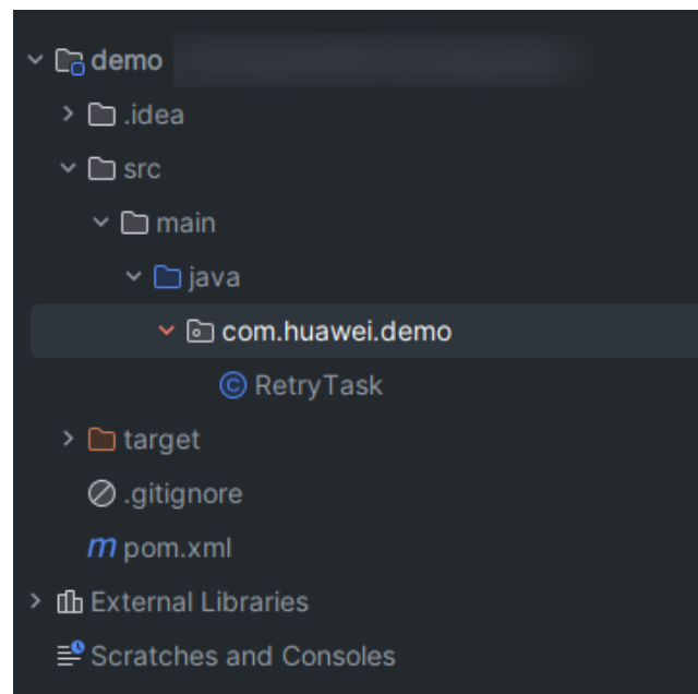
Figure 2-2 Directory structure
